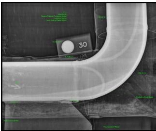
Digital image showing pipe support external corrosion under insulation and solids build-up
