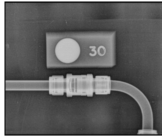
Digital image showing small bore piping fit-up
