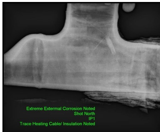
Digital image showing severe external corrosion under insulation
