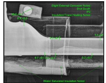
Digital image showing wet insulation and solids build-up
