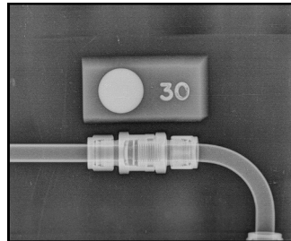
Digital image showing small bore piping fit-up
