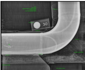
Digital image showing pipe support external corrosion under insulation and solids build-up
